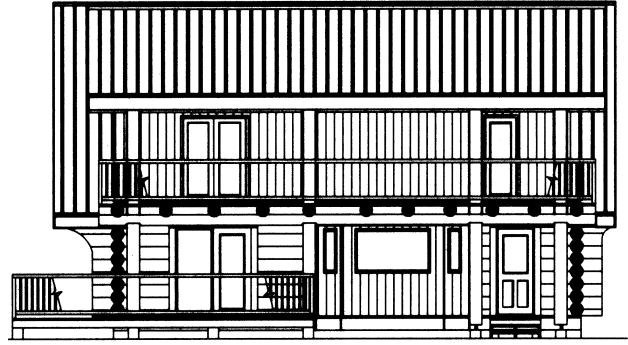
north elevation
